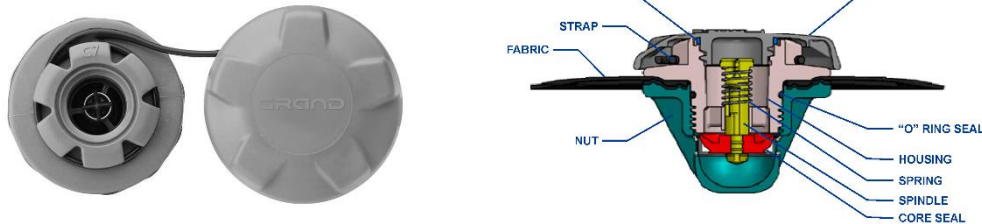
Fig. 14. Inflation valve.
