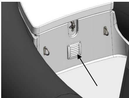
Fig. 6. Ventilation opening on the bow locker.
