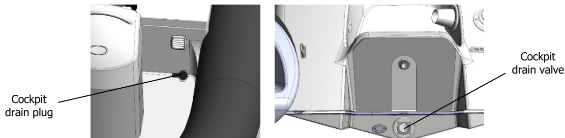
Fig. 2. Cockpit drainage.
