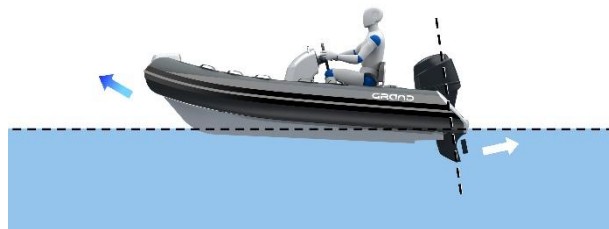
Fig. 20. Trim up.
