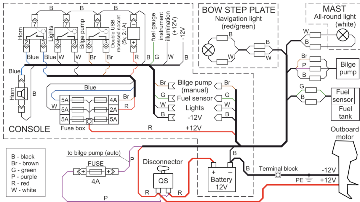
Fig. 47. Electrical schematic diagram of G380.
