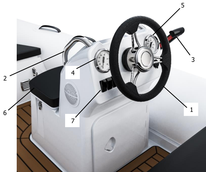
Fig. 43. Steering console components.
