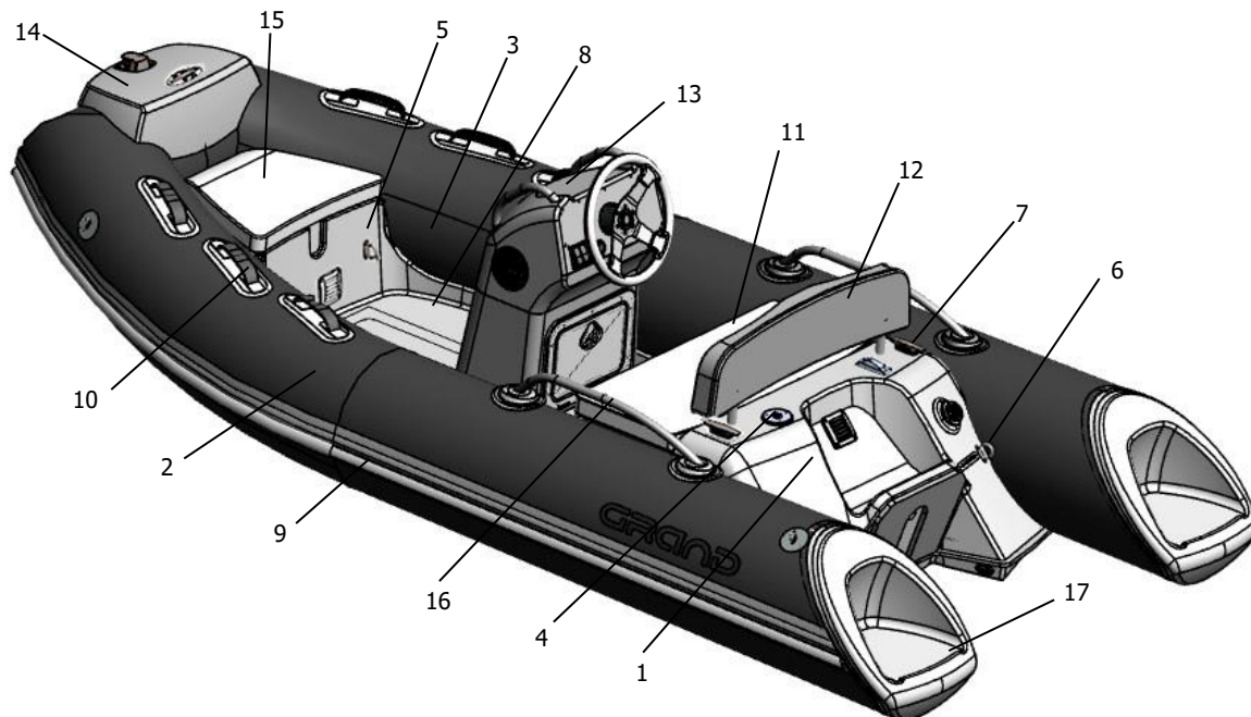
Fig. 42. General arrangement of a boat.
