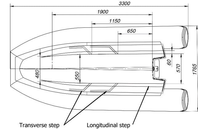
Fig. 49. G340. Measurements for a correct trailer.
