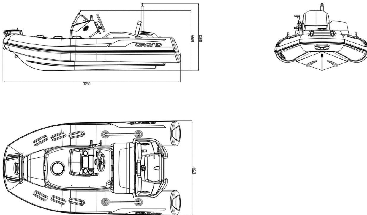
Fig. 47. General view of a boat G340N with single steering console.
