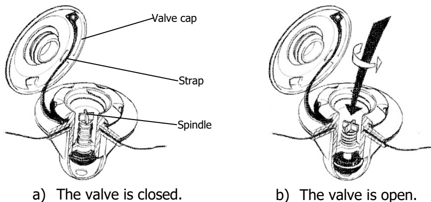
Fig. 14. Design of the inflation valve.
