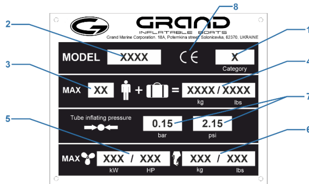
Fig. 6. Builder's plate.
